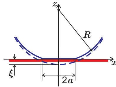
Fig. 1: (Colour on-line) Collision of a visco-elastic sphere of radius R with undeformable plane. Here a is the radius of the contact zone and \xi is the deformation. The contact plane is located at z = 0 .
